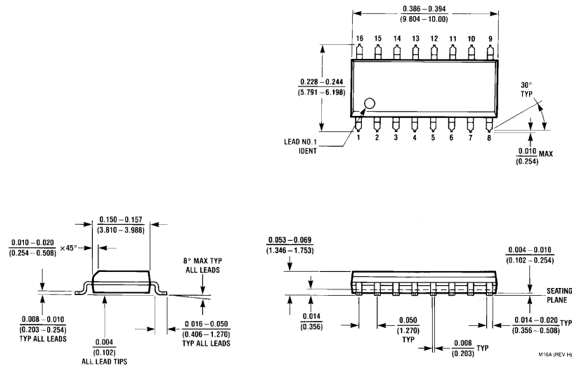
16-Lead (0.150" Wide) Molded Small Outline Package, JEDEC Order Number DM74AS157M or DM74AS158M Package Number M16A
