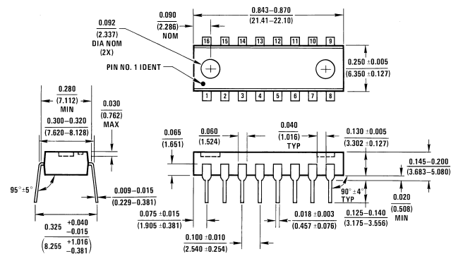
Molded Dual-In-Line Package (N) Order Number DM74AS161N or DM74AS163N Package Number N16A
