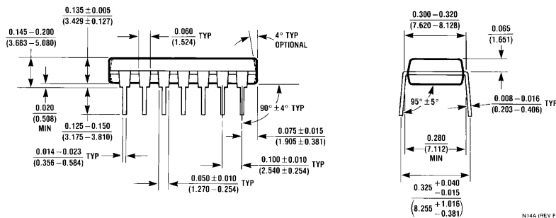
Molded Dual-In-Line Package (N) Order Number DM74AS21N Package Number N14A
