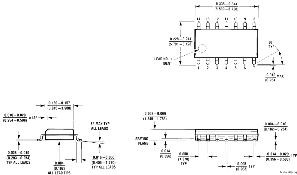
S.O. Package (M) Order Number DM74AS21M Package Number M14A
