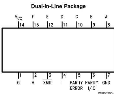
Top View Order Number DM74AS286M or DM74AS286N See Package Number M14A or N14A
