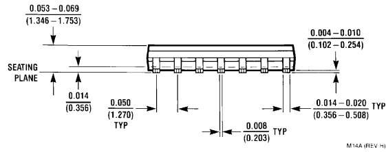
S. O. Package (M) Order Number DM74AS286M Package Number M14A
