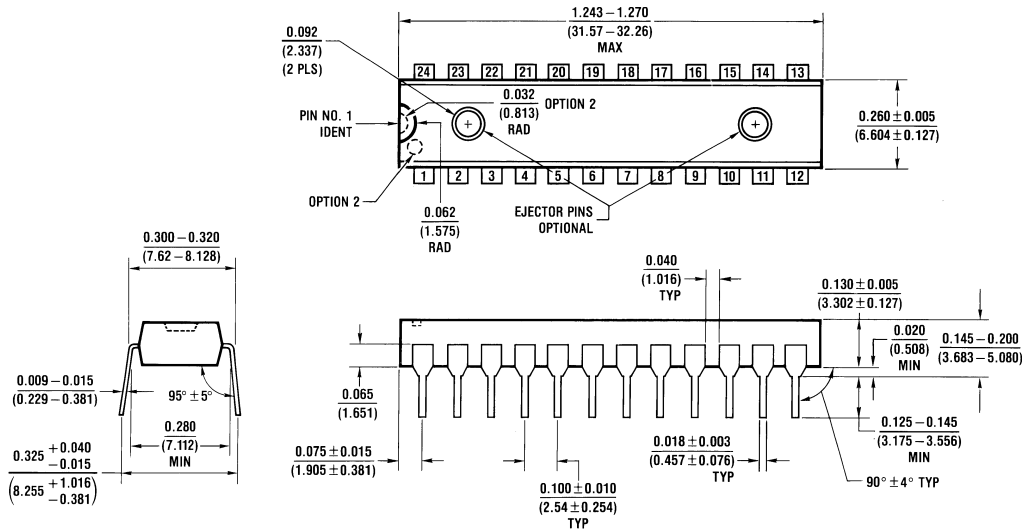
Molded Dual-In-Line Package (N) Order Number DM74AS874NT Package Number N24C
