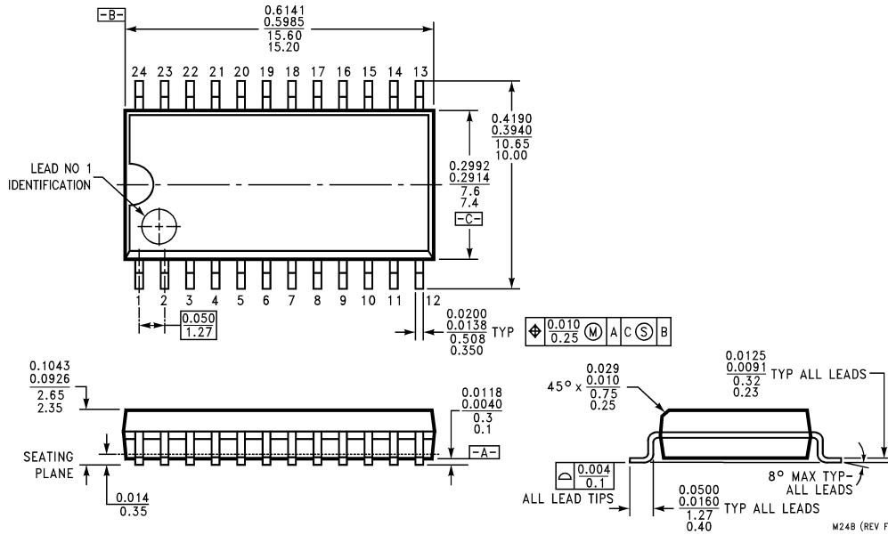
24-Lead (0.300" Wide) Molded Small Outline Package, JEDEC (M) Order Number DM74AS874WM Package Number M24B
