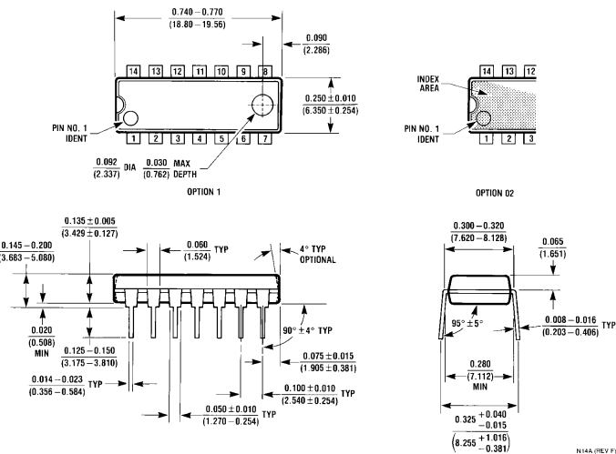
14-Lead Molded Dual-In-Line Package (N) Order Number DM74LS164N Package Number N14A
