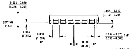
14-Lead Small Outline Molded Package (M) Order Number DM74LS51M Package Number M14A
