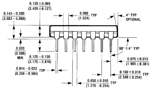
14-Lead Molded Dual-In-Line Package (N) Order Number DM74LS51N Package Number N14A
