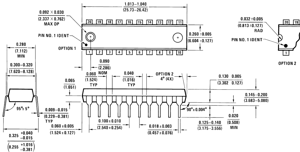
20-Lead Molded Dual-In-Line Package (N) Order Number DM74LS574N Package Number N20A
