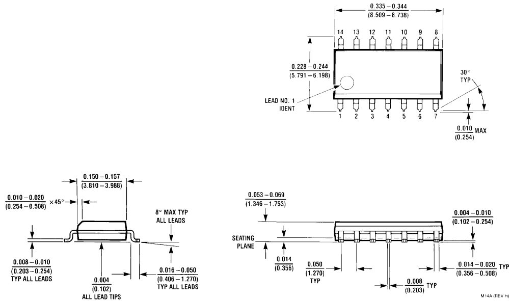
14-Lead Small Outline Molded Package (M) Order Number DM74S280M Package Number M14A
