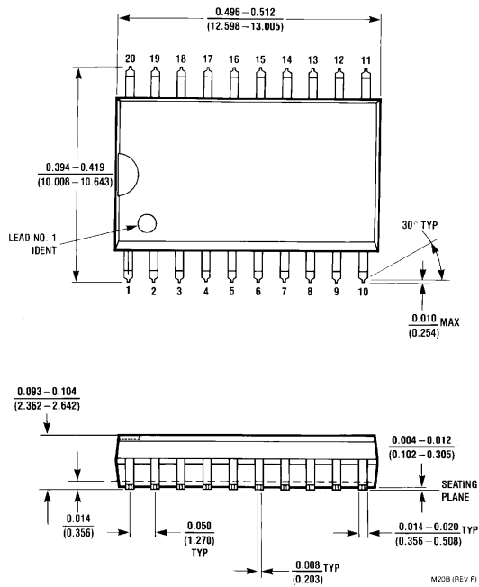
20-Lead Wide Small Outline Molded Package (M) Order Number DM74S373WM or DM74S374WM Package Number M20B
