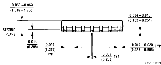
14-Lead Small Outline Molded Package (M) Order Number DM74S74M Package Number M14A
