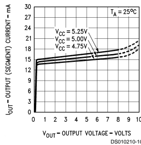
FIGURE 2. Typical Constant Segment Current Versus Output Voltage
