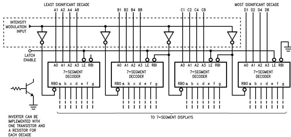
FIGURE 4. Intensity Control by \overline{\text{RBO}} Pulse Duty Cycle
