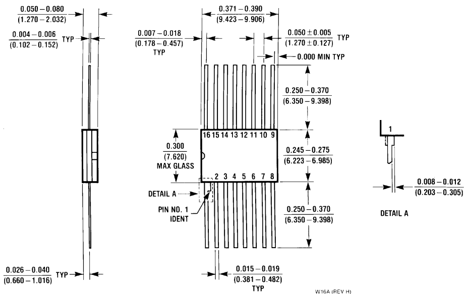
16-Lead Ceramic Flat Package (W) Order Number 96LS02FMQB Package Number W16A
