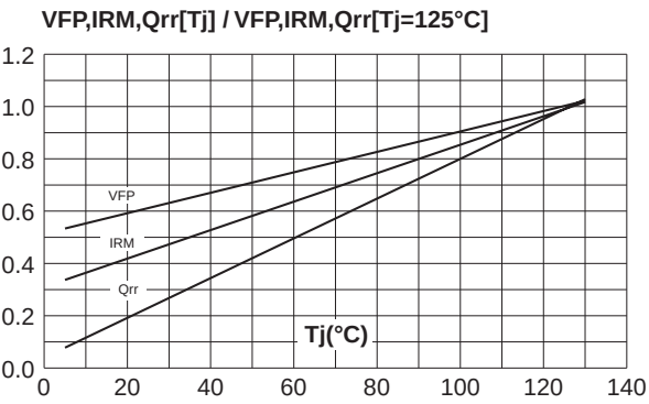
Fig. 10-1: Dynamic parameters versus junction temperature (damper diode).
