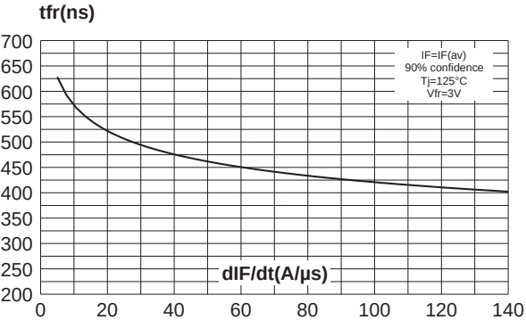
Fig. 9-1: Forward recovery time versus diF/dt (damper diode).
