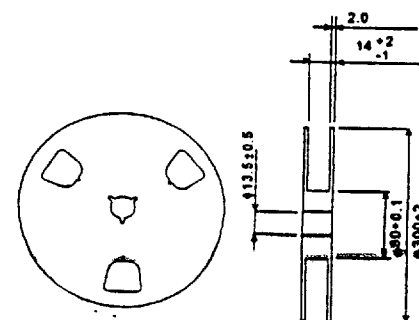
330 mm/13" Reel
