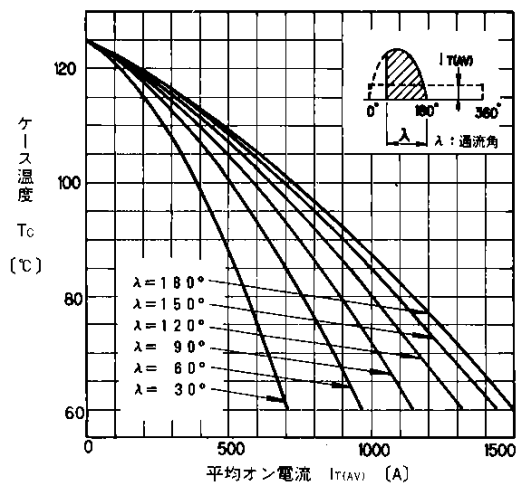
T_c - I_{T(AV)} Characteristics (Sine Wave)
