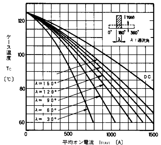
T_c - I_{T(AV)} Characteristics (Square Wave)
