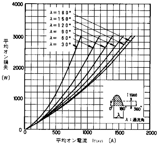
Average On-state Loss (Sine Wave Current)
