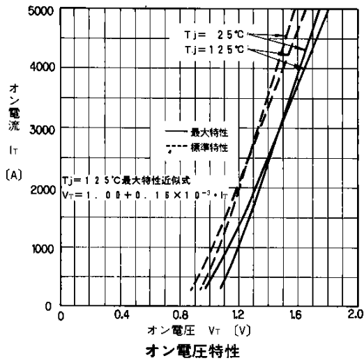
On-state Characteristics
