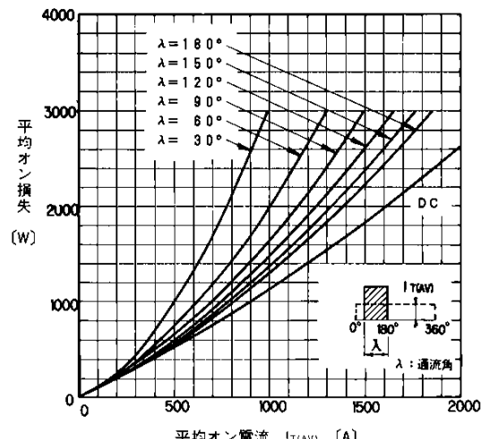
Average On-state Loss (Square Wave Current)
