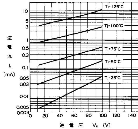
Reverse Characteristics
