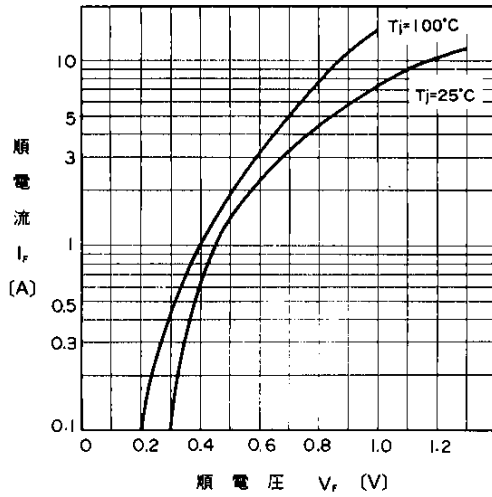
Forward Characteristics
