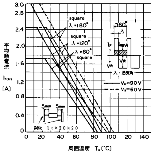
I_{F(AV)}-T_a Characteristics
