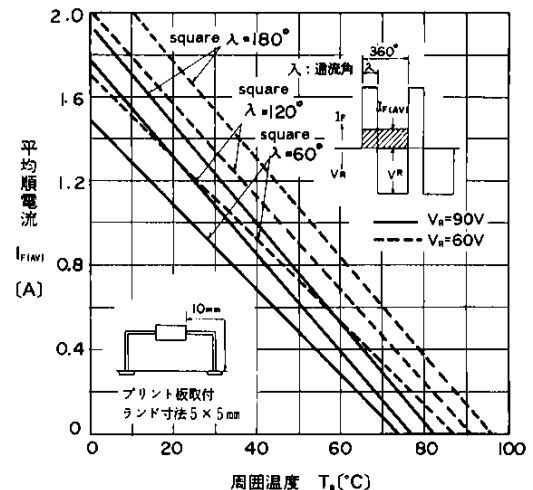
I_{F(AV)}-T_a Characteristics
