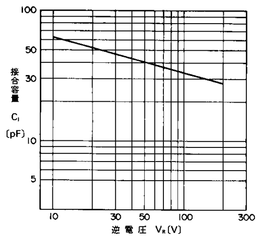
接合容量特性 Junction Capacitance Characteristics
