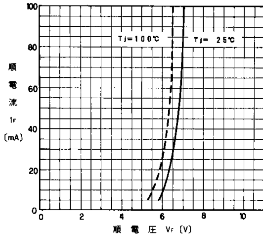
順特性 (代表特性) Forward Characteristics
