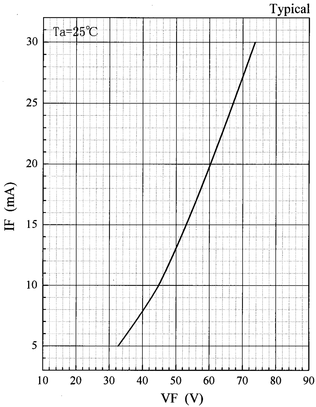
Fig.1 Forward characteristic[VF-IF]
