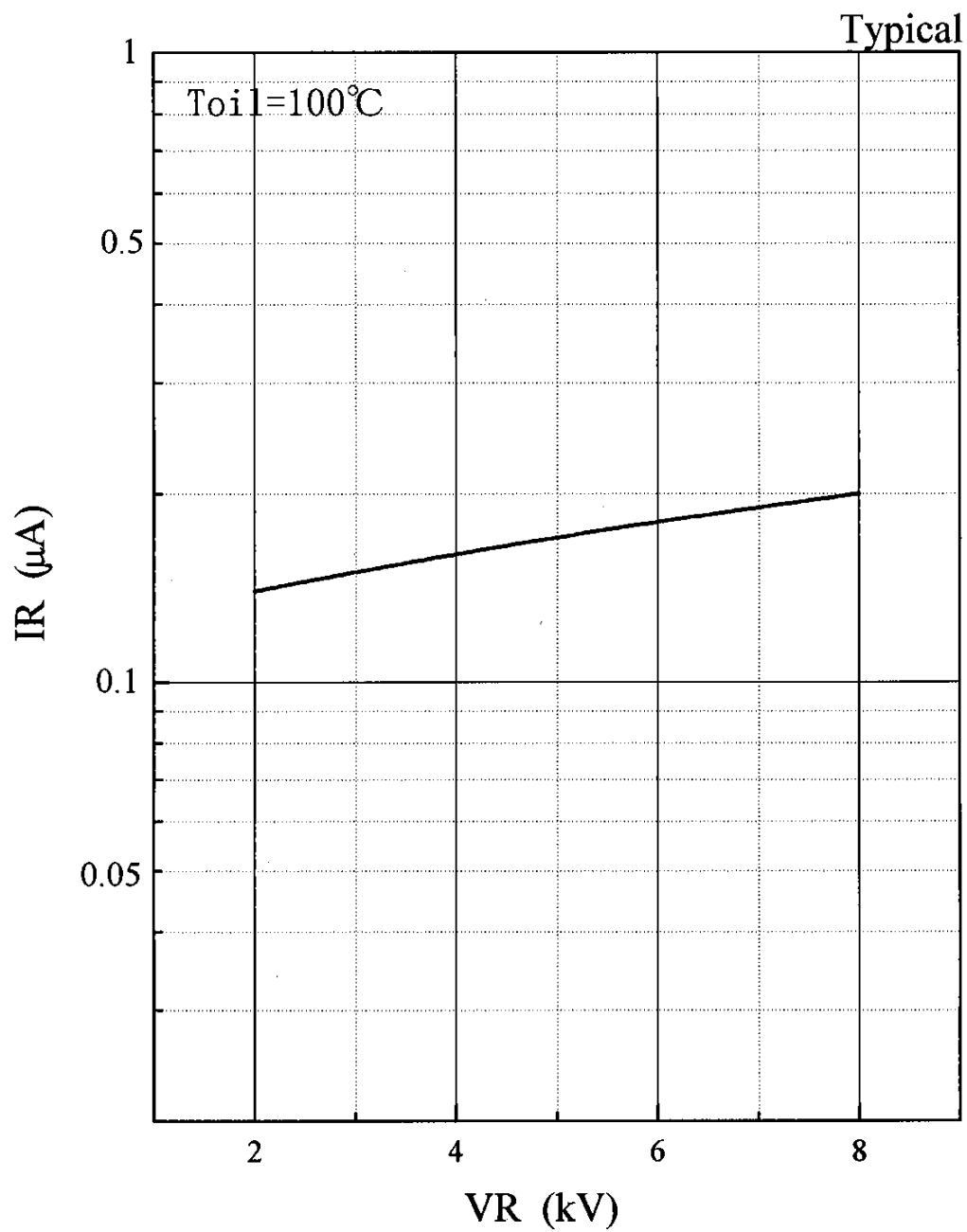
Fig.2 Reverse characteristic[VR-IR]
