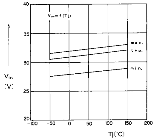
Over-Voltage Detection
