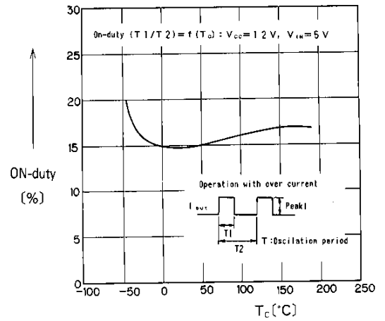
Over-Current protection
