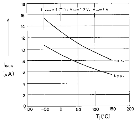
Input Current
