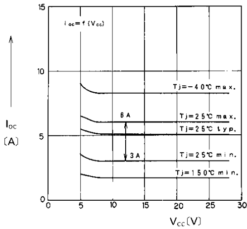
Over-Current Detection
