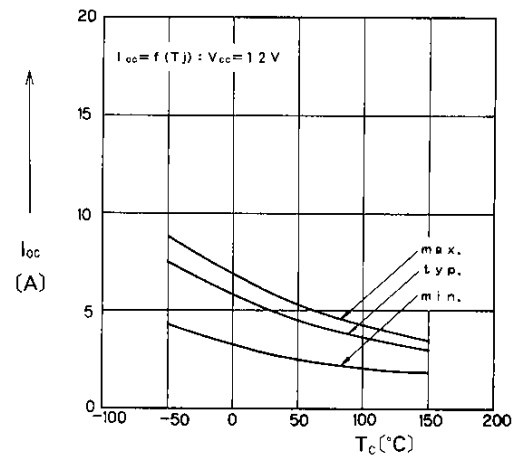
Over-Current Detection
