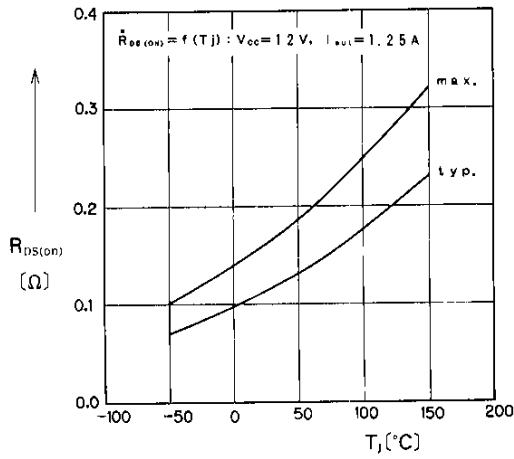
On-Stage Resistance
