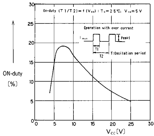
Over-Current protection
