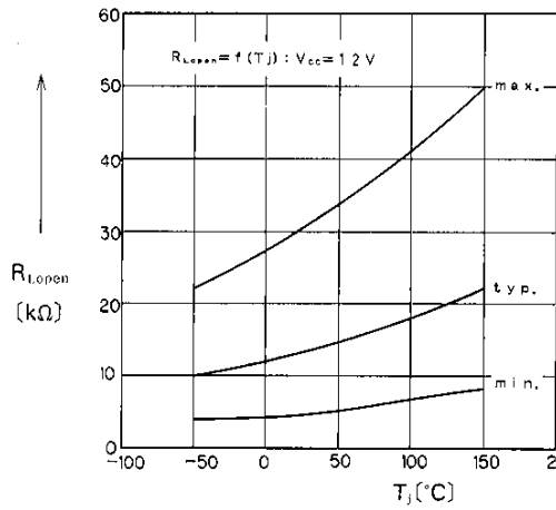
Open-Load Detection
