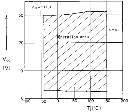
Operation Voltage
