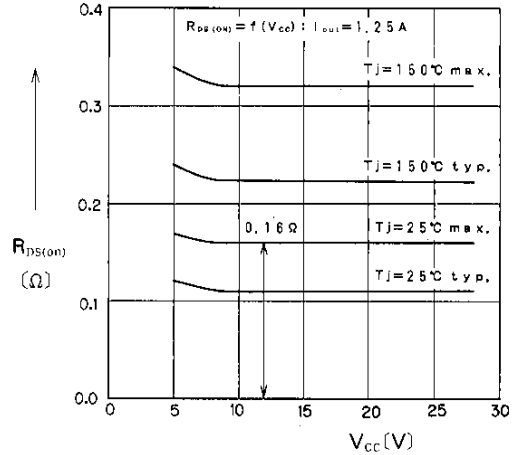
On-State Resistance
