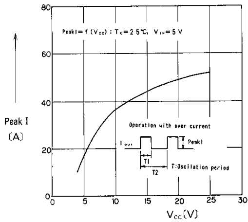
Over-Current protection
