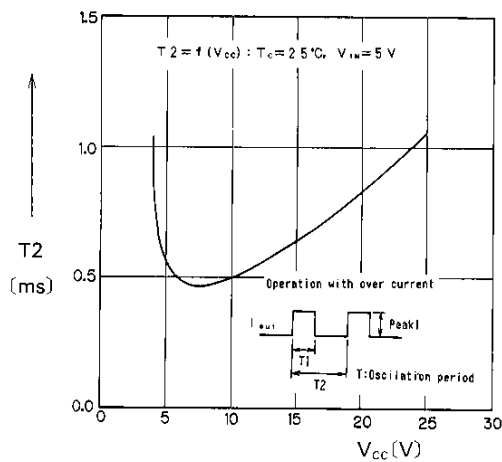
Over-Current protection
