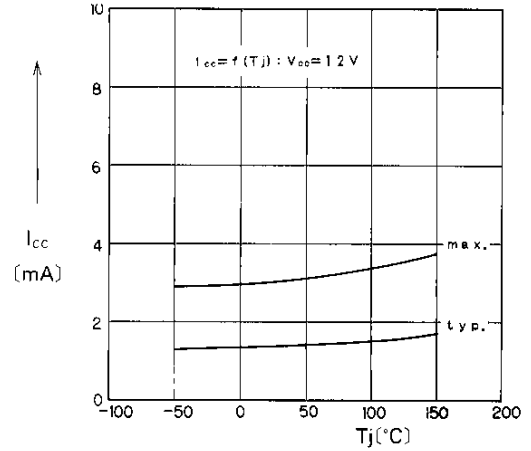
Standby Current
