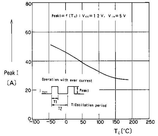
Over-Current Protection
