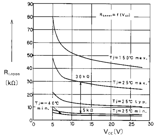
Open-Load Detection
