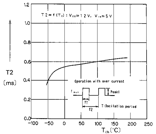
Over-Current Protection
