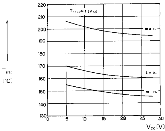
Over-Temperature Detection
