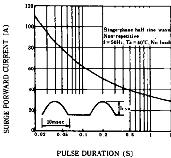
FIG.4-SURGE CURRENT RATINGS
