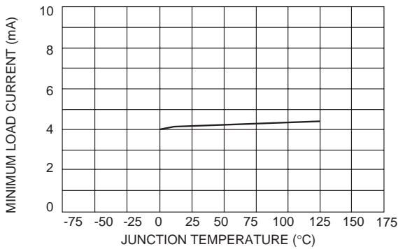
Mimimum Load Current vs. Temperature
