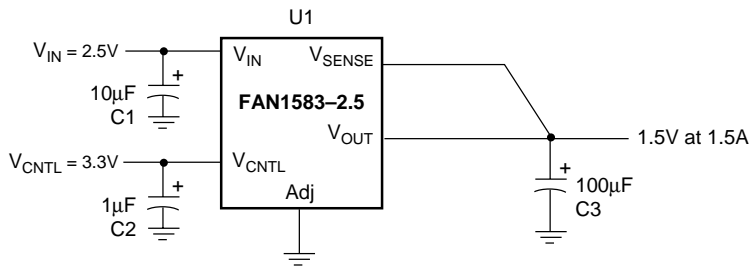
Figure 5. Application Circuit (FAN1583-2.5)
