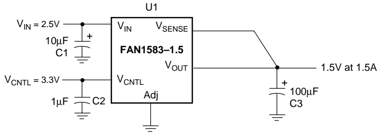
Figure 4. Application Circuit (FAN1583-1.5)
