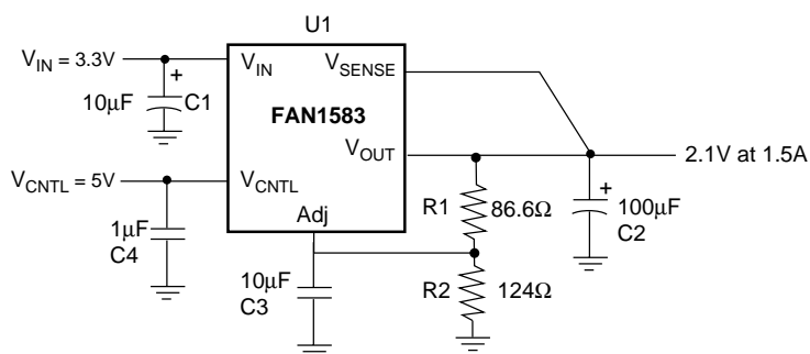
Figure 3. Application Circuit (FAN1583)
