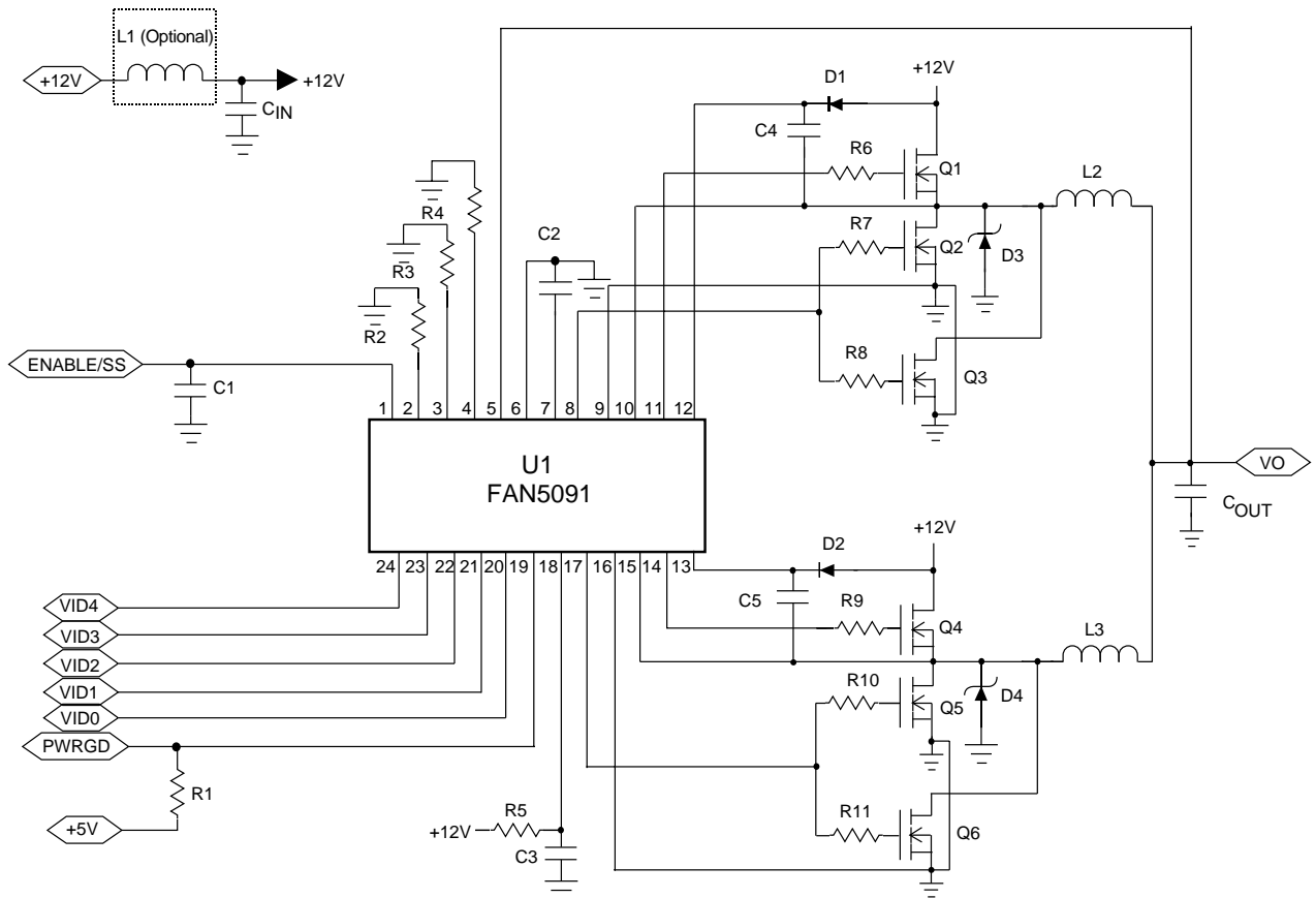
Figure 1. Application Circuit for +12V Power, 50A Low Frequency Application (300 MHz each slice)
