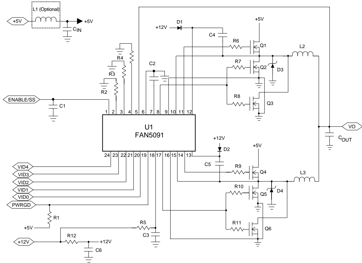
Figure 2. Application Circuit for +5V Power, 40A High Frequency Application (1MHz each slice)
