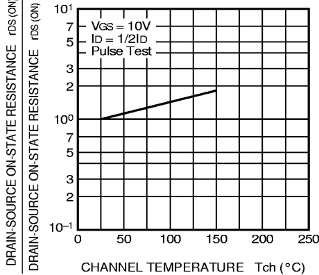
ON-STATE RESISTANCE VS. CHANNEL TEMPERATURE (TYPICAL)
