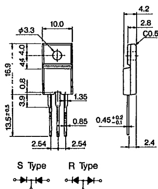
Outline Drawing 62
