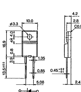
Outline Drawing 64
