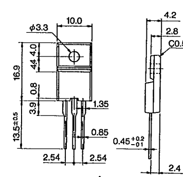
Outline Drawing ④8
