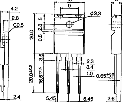
Outline Drawing ④8
