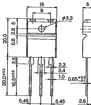
Outline Drawing ④8
