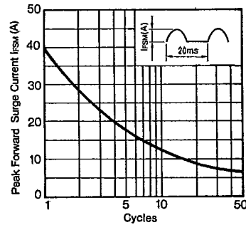
I_FSM Characteristics
