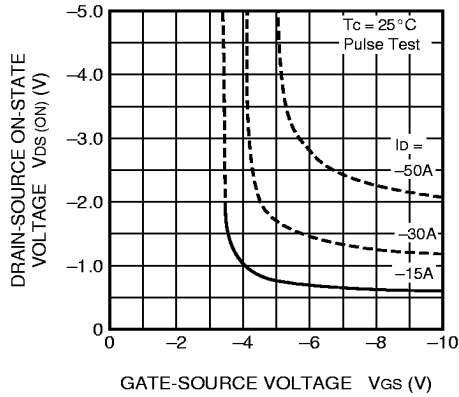
ON-STATE VOLTAGE VS. GATE-SOURCE VOLTAGE (TYPICAL)
