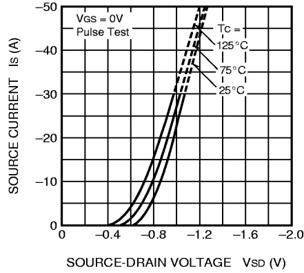
SOURCE-DRAIN DIODE FORWARD CHARACTERISTICS (TYPICAL)
