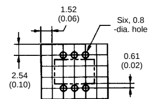
PCB Dimensions (Bottom View)
