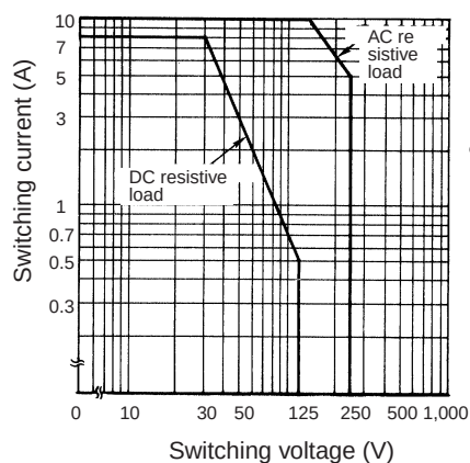
Maximum Switching Power G5LC
