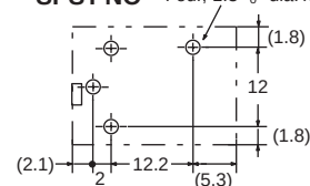
SPST-NO
