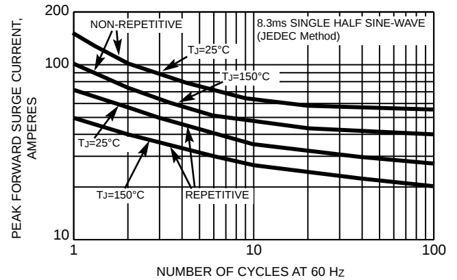
FIG. 2 - MAXIMUM PEAK FORWARD SURGE CURRENT
