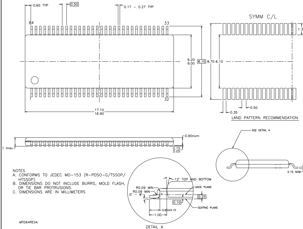
64-Lead Thin Shrink Small Outline Package, JEDEC MO-153, 6.1mm Wide Package Number MTD64
