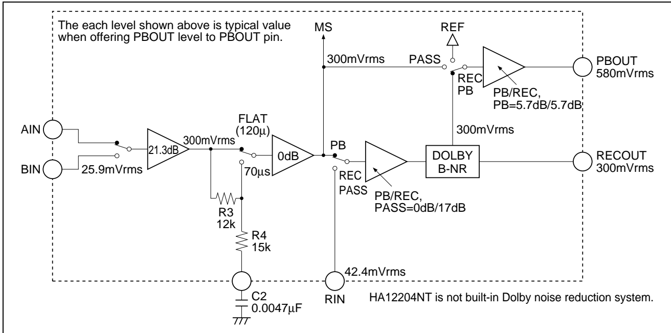
Figure 2 Input Block Diagram
