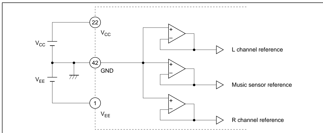
Figure 1 Reference Voltage
