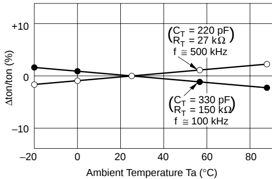
\Delta \text{ton/ton} vs. Ambient Temperature (HA16654A)
