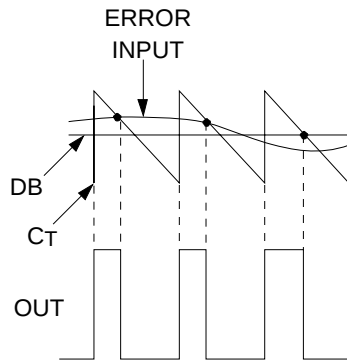
Figure 1 Waveform Timing
