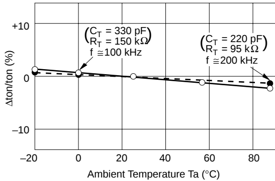
\Delta \text{ton/ton} vs. Ambient Temperature (HA16664A)
