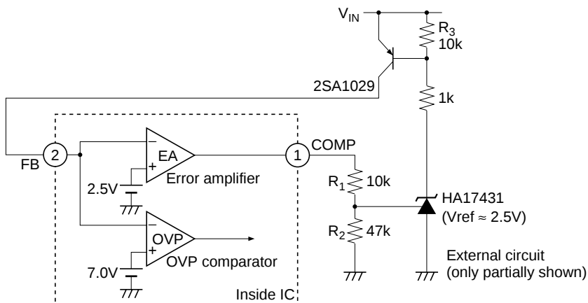
Figure 15 Example of OVP Latch Application Circuit
