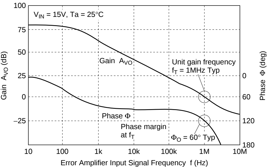
Figure 10 Open Loop Gain Characteristics of Error Amplifier
