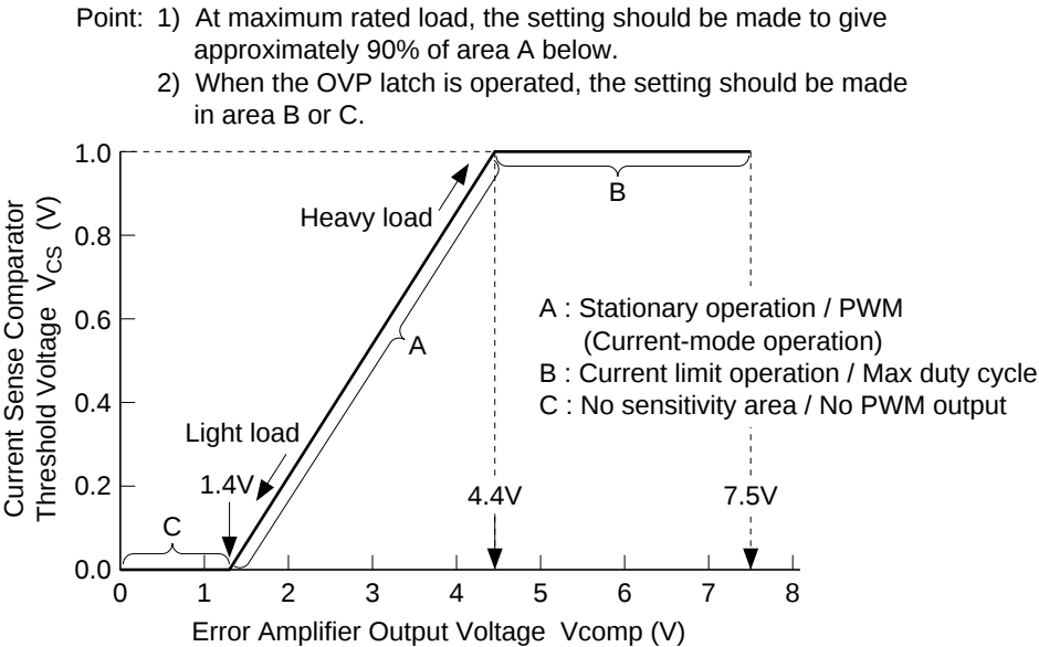
Figure 4 Current Sense Characteristics
