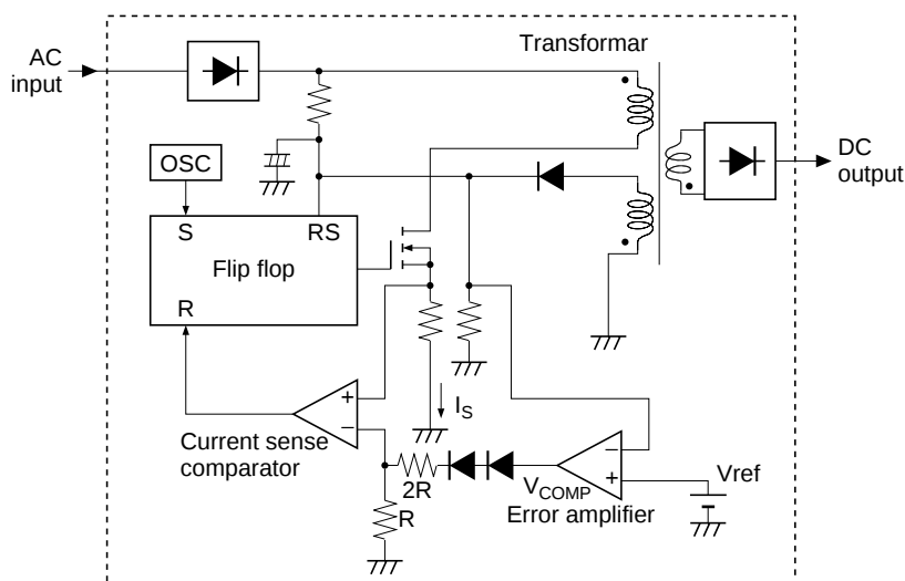
Figure 5 Block Diagram of Current Mode Switching Power Supply
