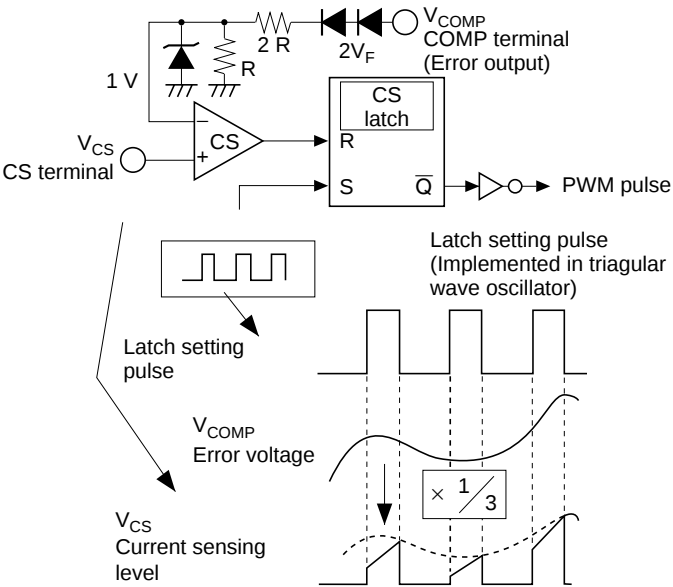
Figure 3 Operation Diagram of Current Sensing Part
