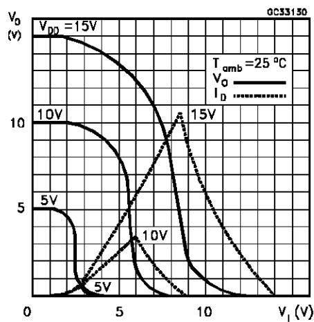
Typical Current and Voltage Transfer Characteristics for Inverter and Test Circuit
