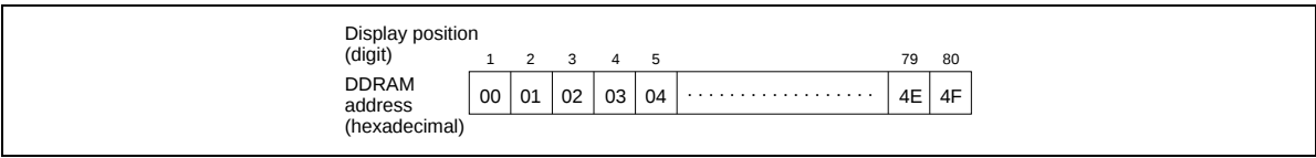
Figure 2 1-Line Display
