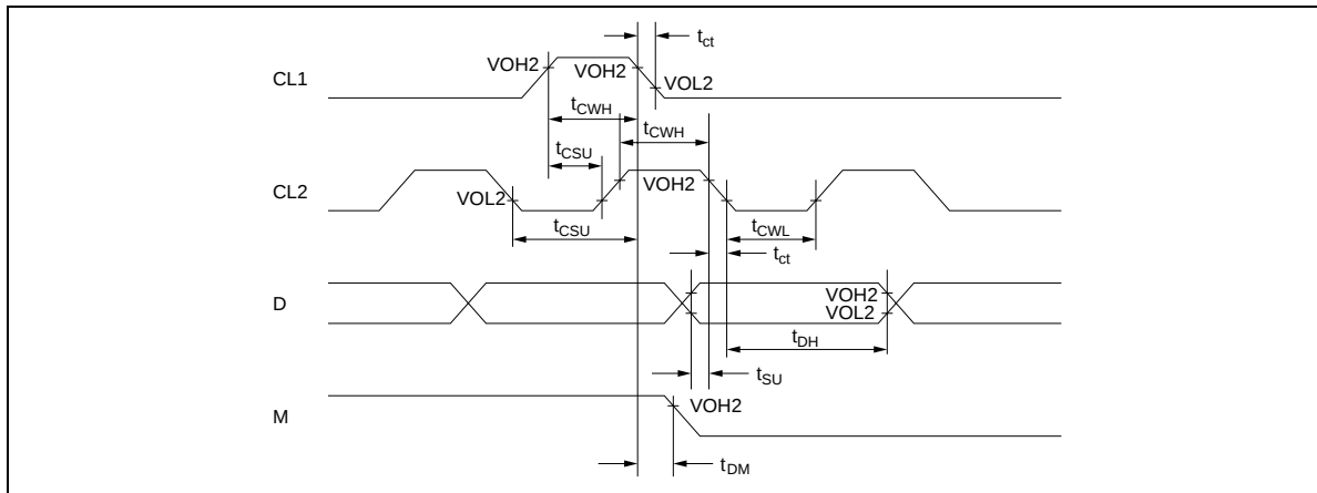
Figure 29 Interface Timing with External Driver
