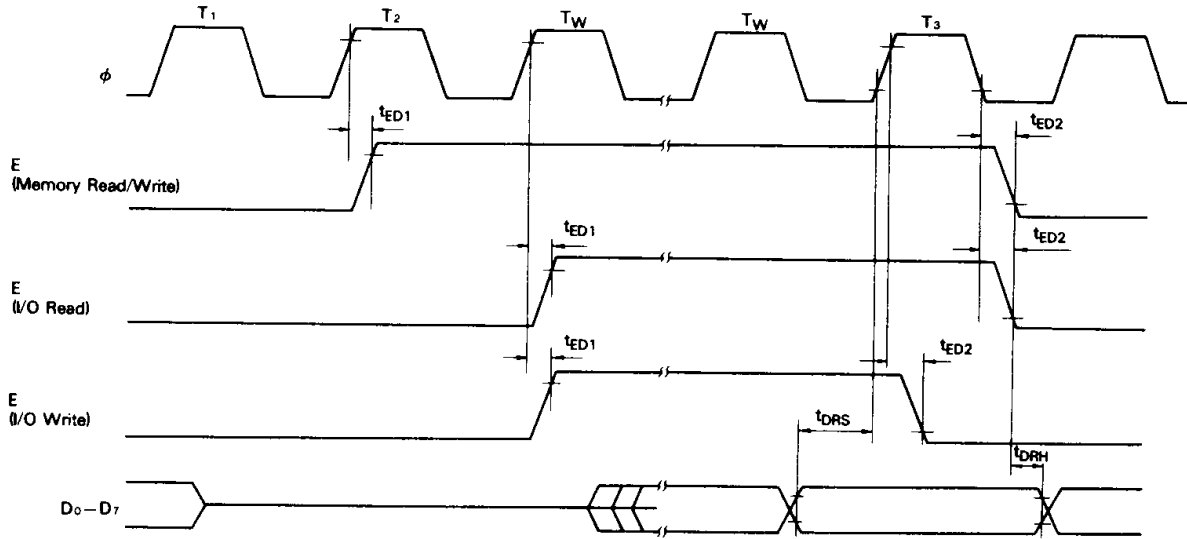
Figure 3 E Clock Timing (1)
