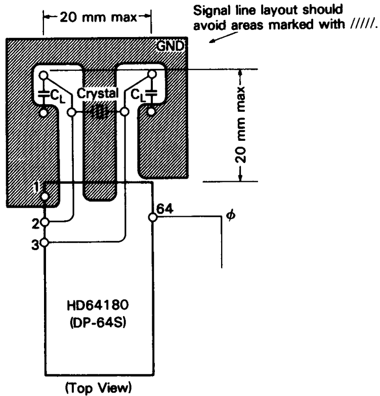
Figure 67 Example of Board Design
