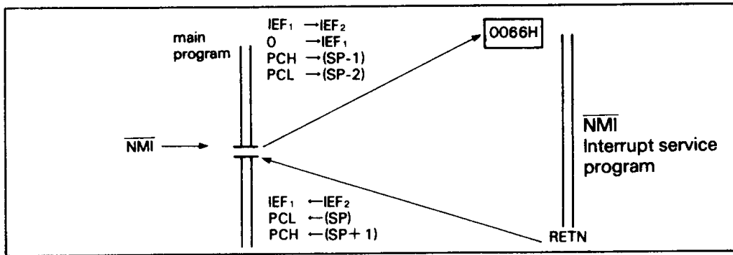
Figure 22 \overline{\text{NMI}} Sequence
