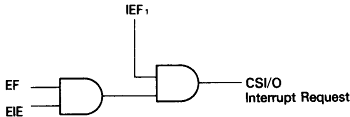
Figure 52 CSI/O Interrupt Circuit Diagram
