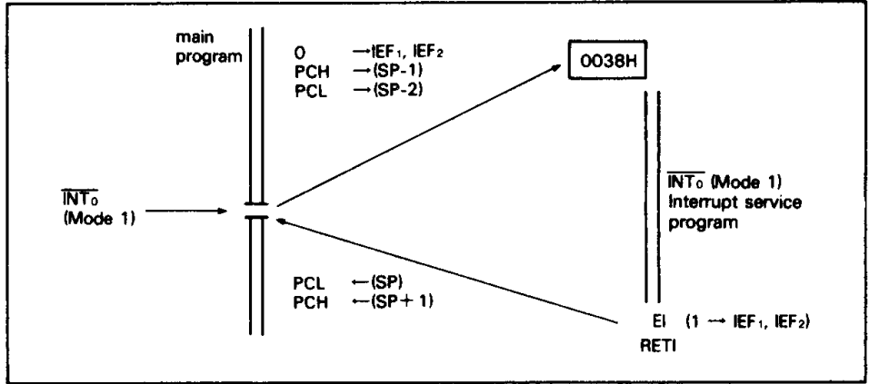
Figure 25 INT 0 Mode 1 Interrupt Sequence
