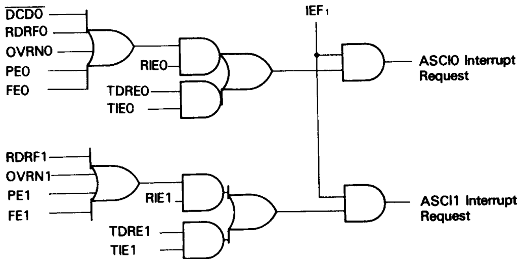
Figure 49 ASCI Interrupt Request Circuit Diagram
