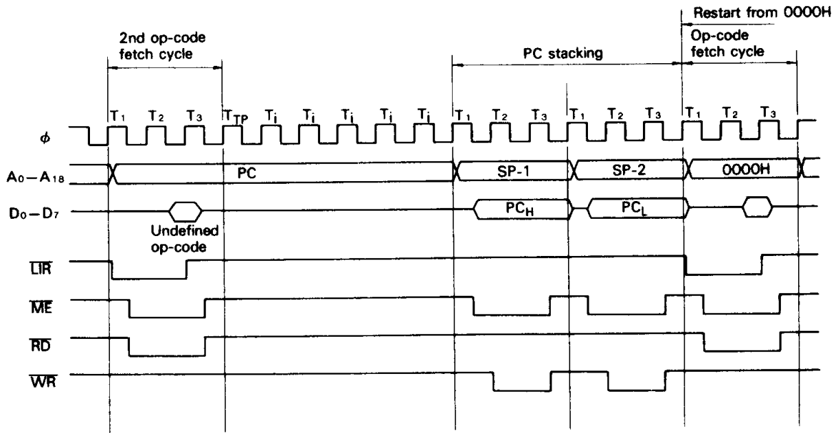
Figure 21 (a) TRAP Timing – 2nd Op-code Undefined
