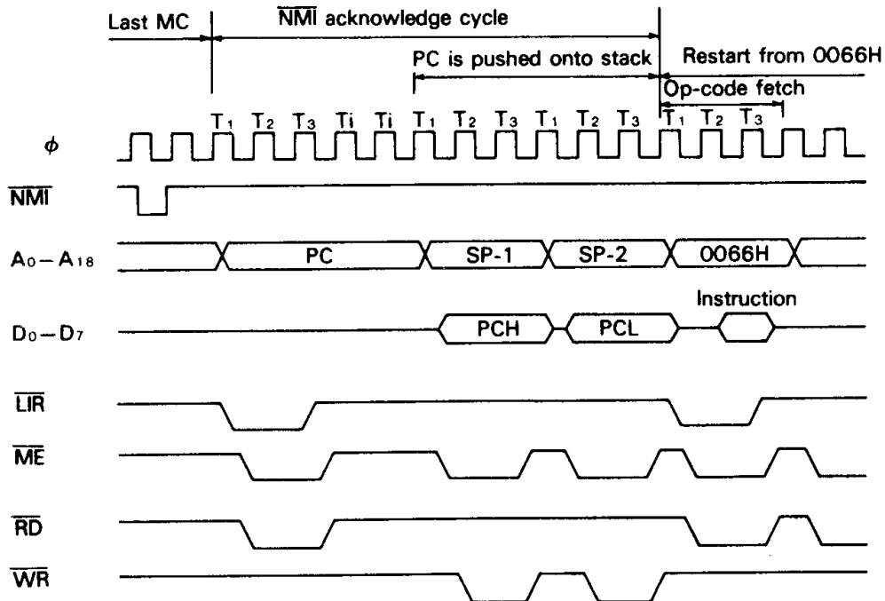
Figure 23 \overline{\text{NMI}} Timing
