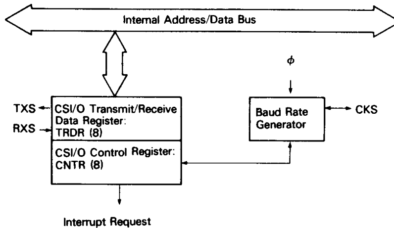
Figure 51 CSI/O Block Diagram
