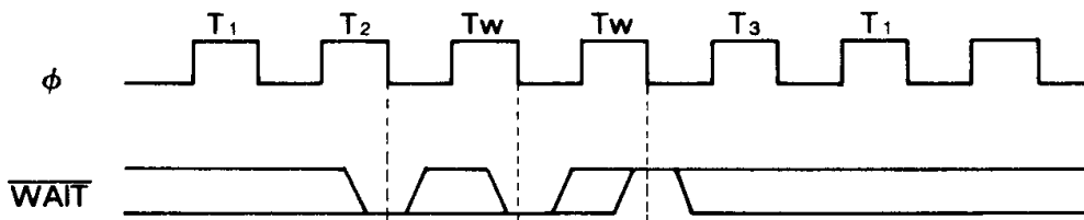
Figure 39 \overline{\text{WAIT}} Timing
