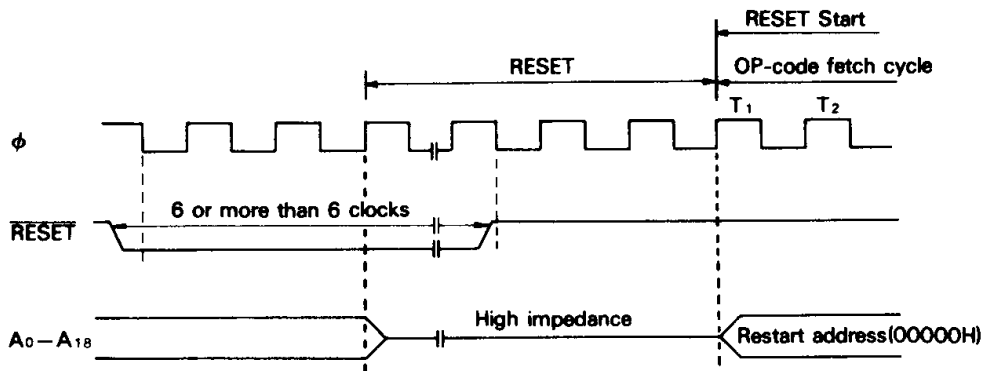
Figure 15 RESET Timing
