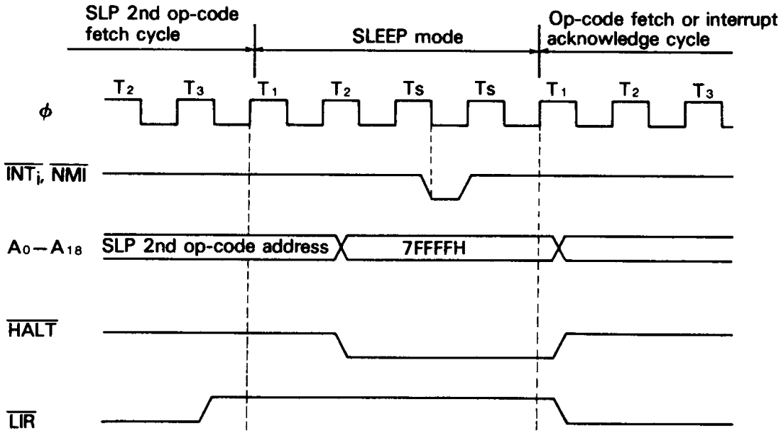
Figure 19 SLEEP Timing
