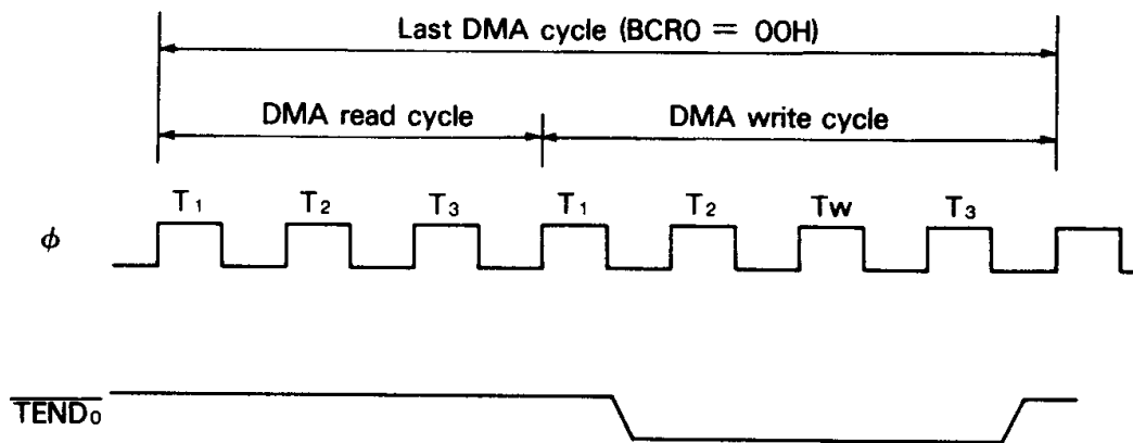
Figure 44 \overline{TEND}_0 Output Timing
