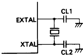
Figure 65 Crystal Interface
