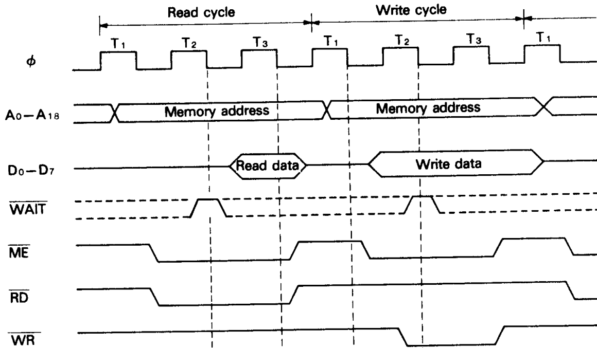
Figure 11 Memory Read/Write Timing (without wait state)
