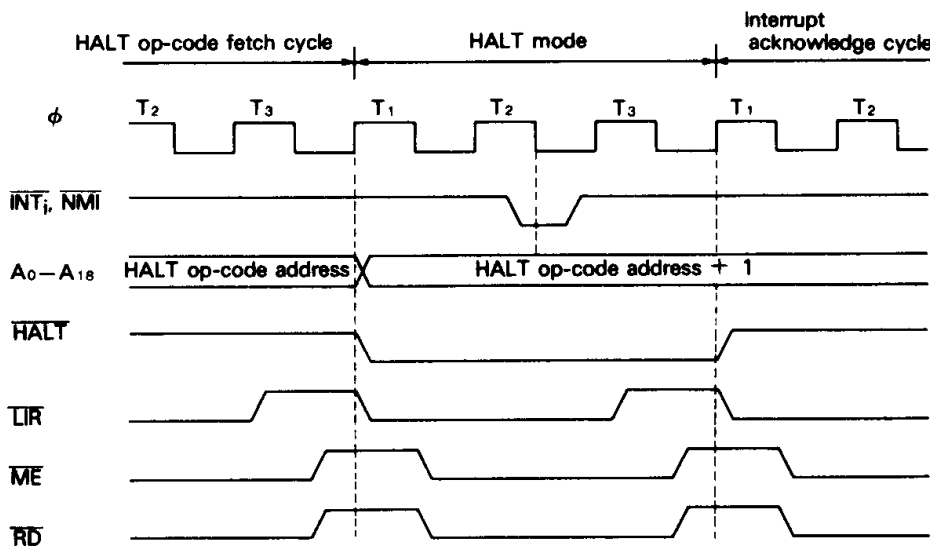
Figure 18 HALT Timing
