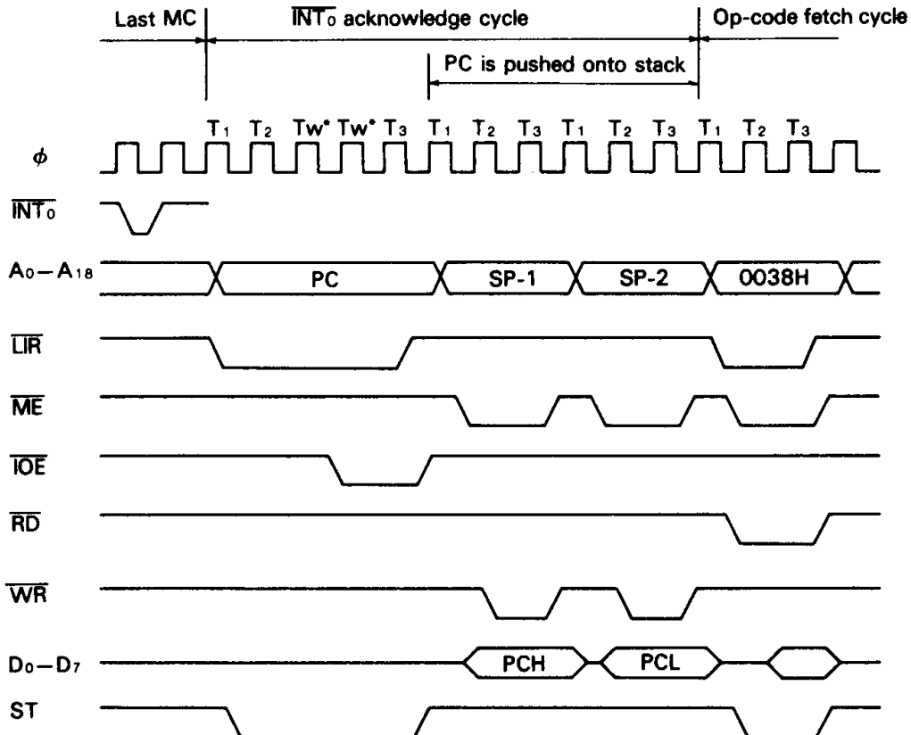
Figure 26 INT 0 Mode 1 Timing
