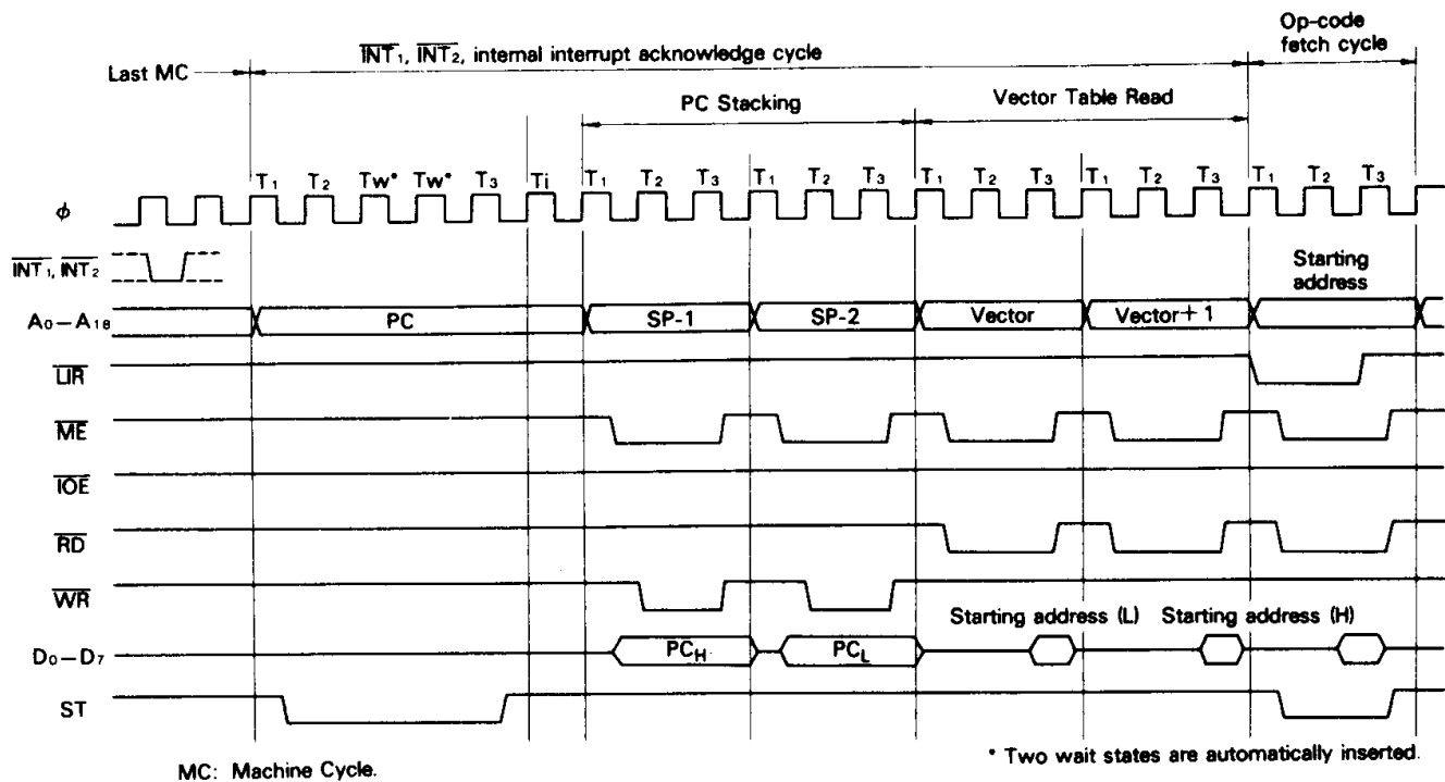
Figure 30 \overline{INT}_1, \overline{INT}_2 and Internal Interrupts Timing
