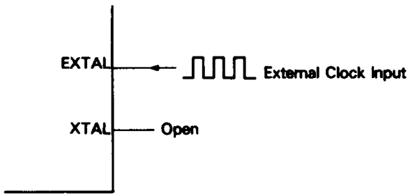
Figure 64 External Clock Interface
