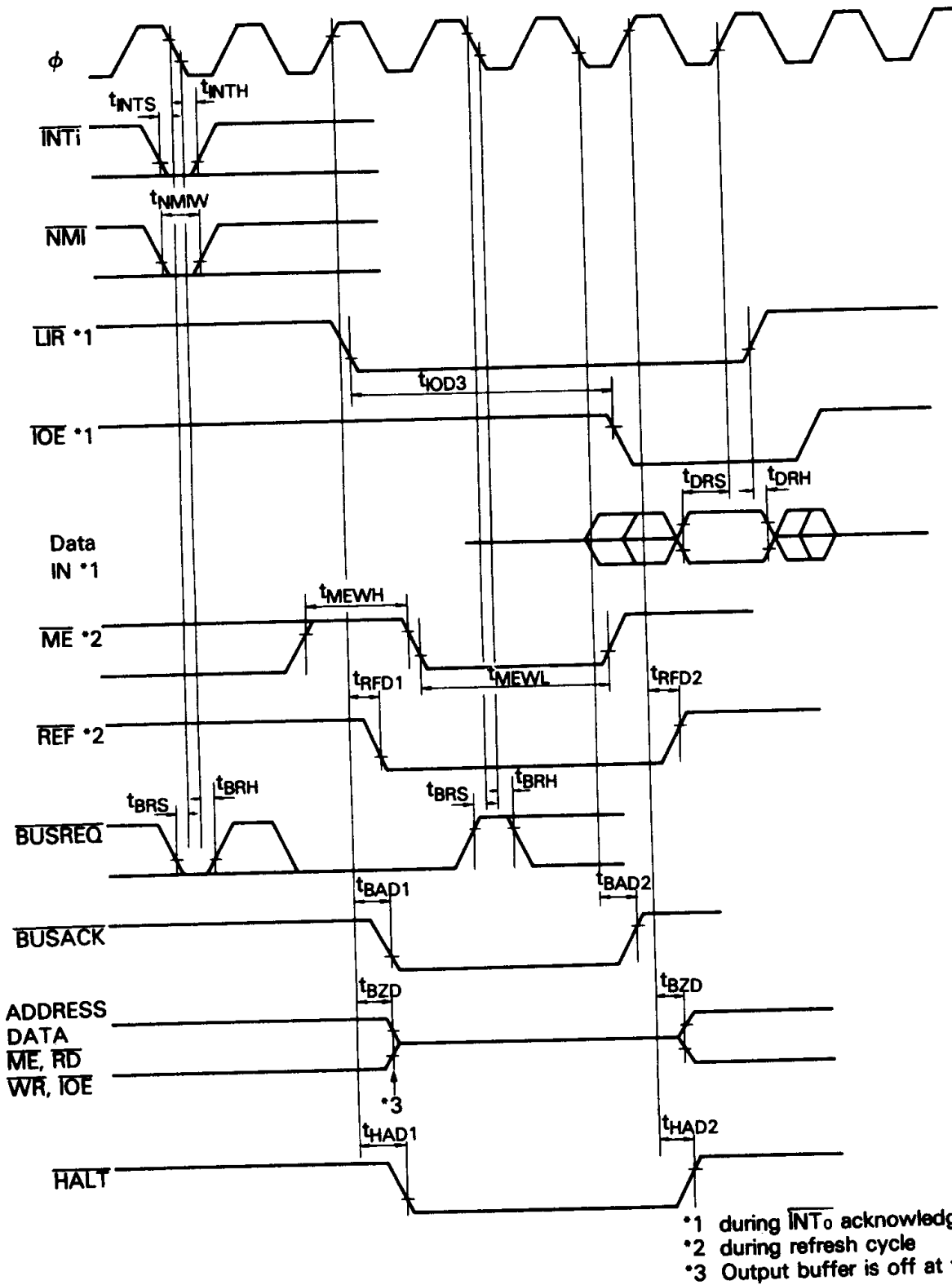
Figure 1 CPU Timing (2)
