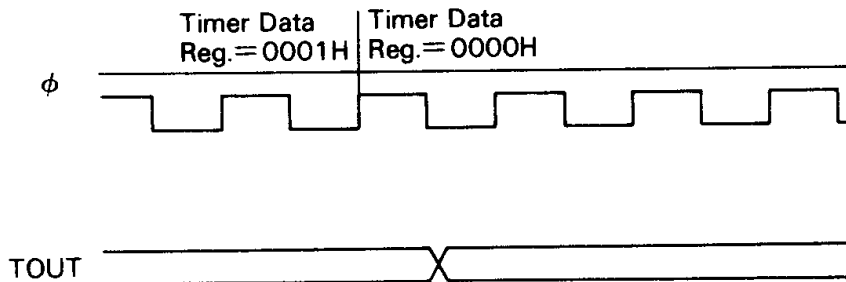
Figure 59 PRT Output Timing
