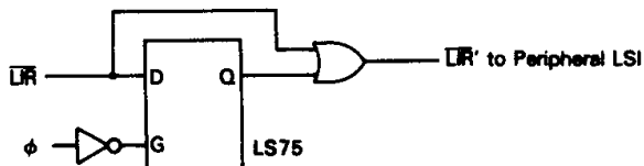
Figure 72 Circuit Example
