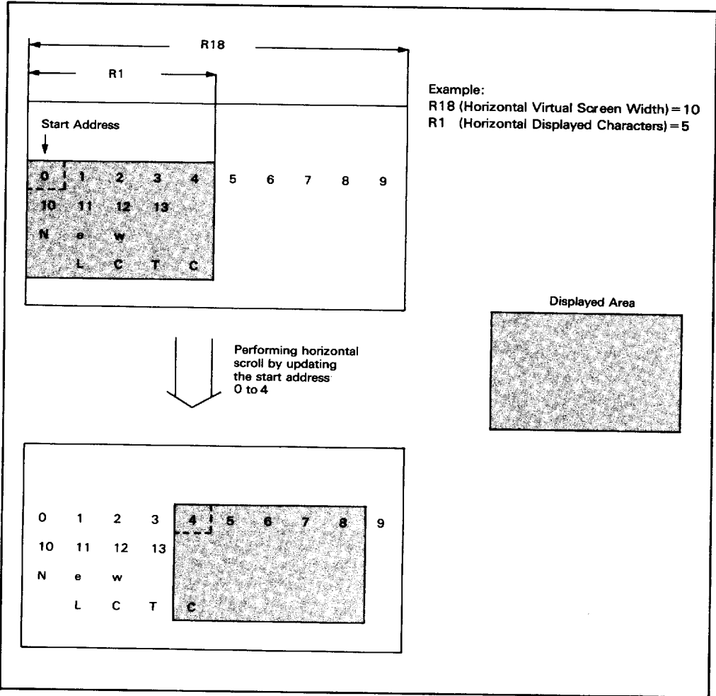
Figure 14 Example of Horizontal Scroll by Setting Horizontal Virtual Screen Width
