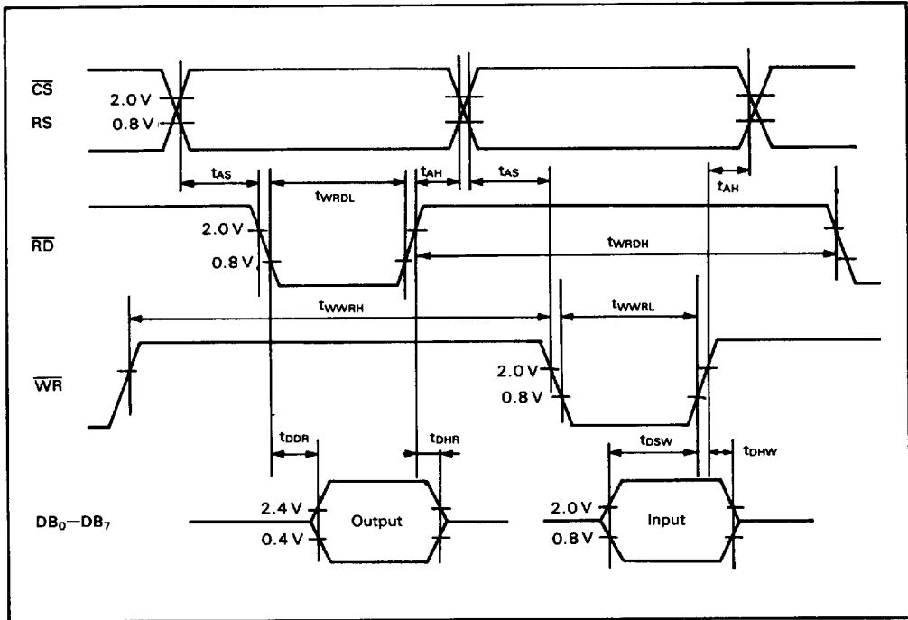
Figure 38 CPU Interface (HD64645 and HD64646)
