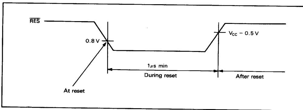
Figure 36 Reset Definition
