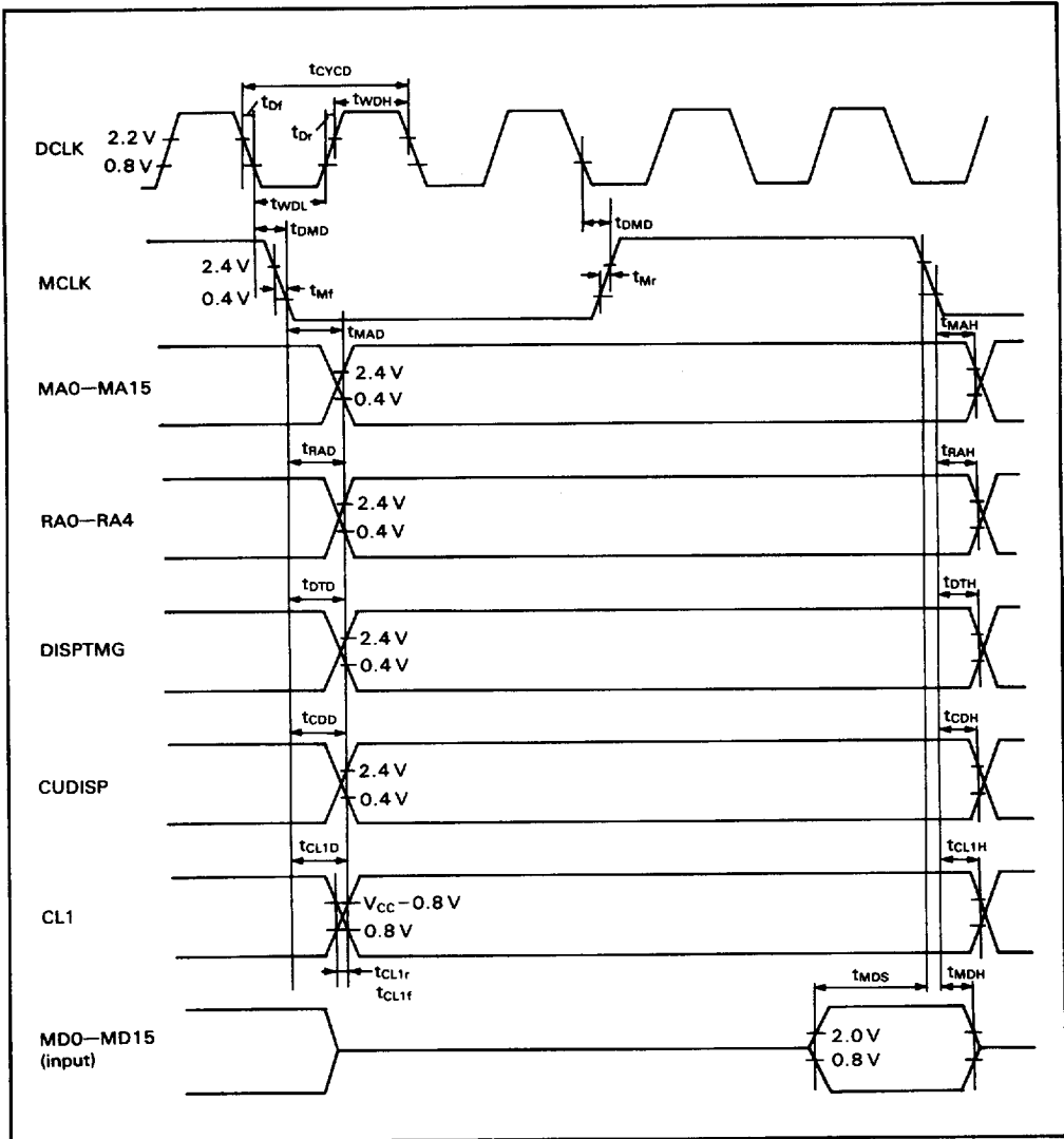
Figure 39 Memory Interface
