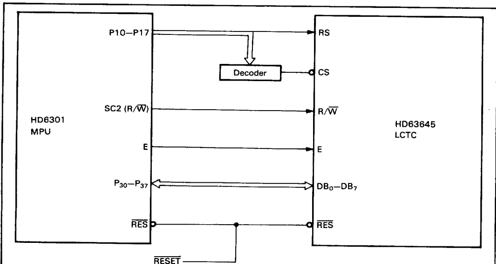
Interface between HD6301 and HD63645
