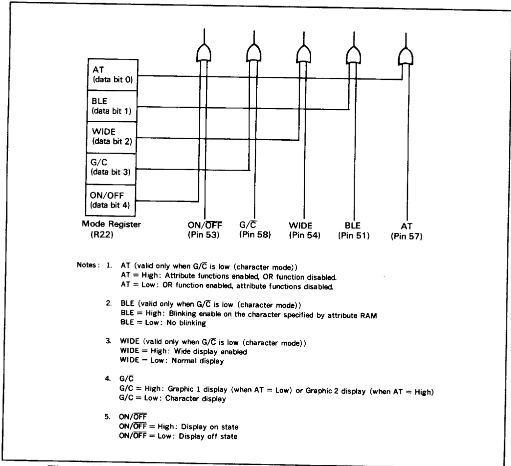
Figure 35 Correspondence between Mode Register and External Pins
