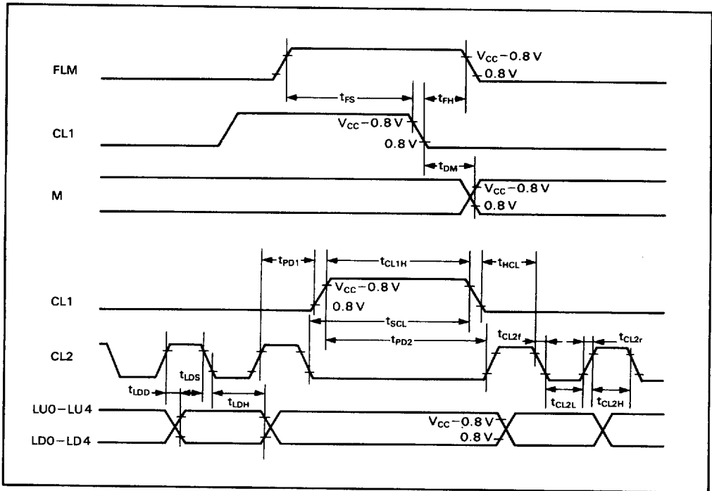
Figure 41 LCD Interface
