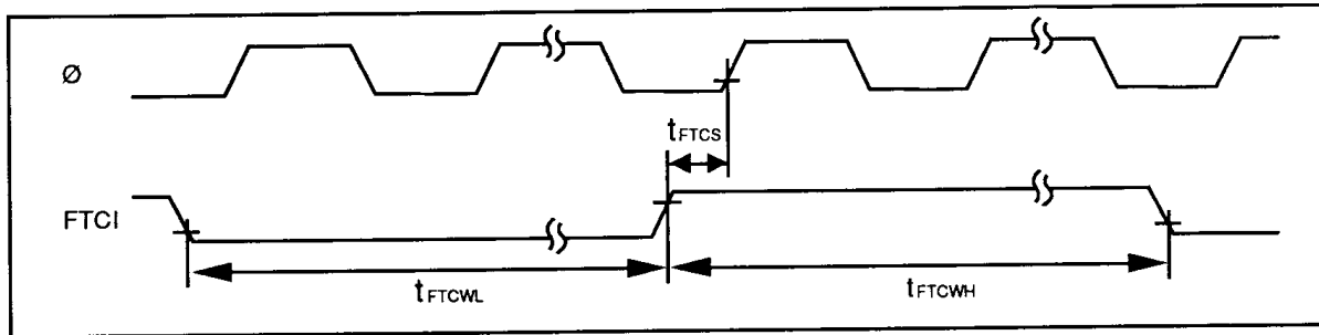
Figure 15-12. External Clock Input Timing for Free-Running Timer
