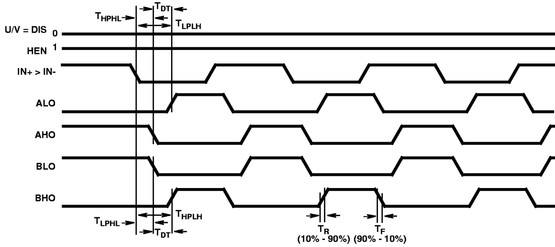
FIGURE 1. BISTATE MODE
