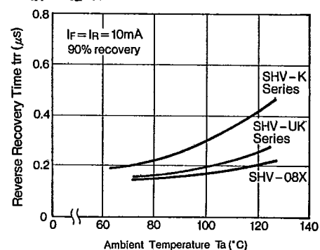
trr - ta Characteristics
