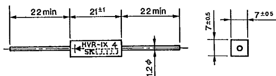
Outline Drawing ③⑪
