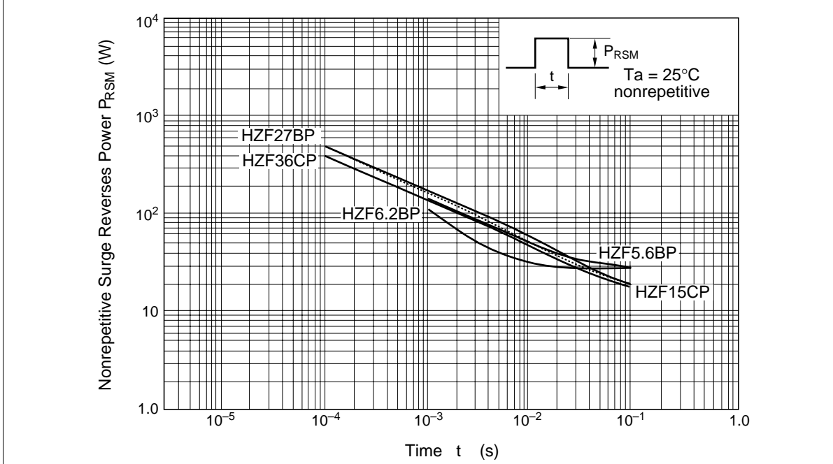
Fig.4 Surge Reverse Power Ratings (Reference only)
