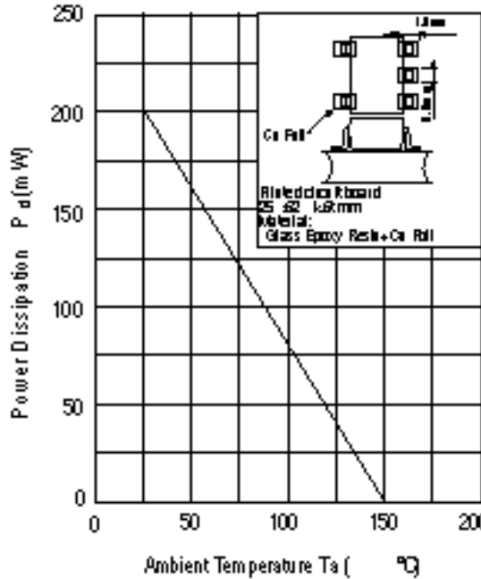
Fig.2 Power Dissipation Vs. Ambient Temperature
