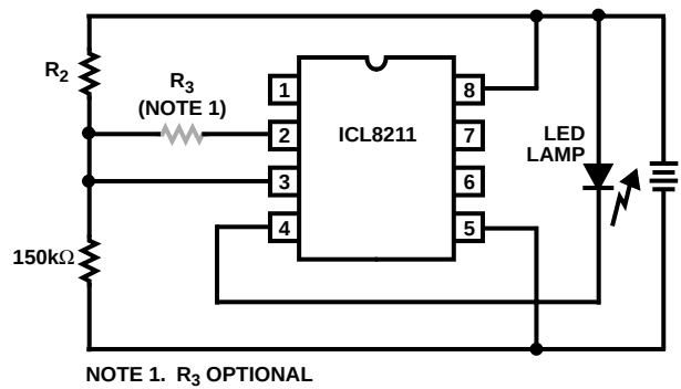
FIGURE 28. LOW VOLTAGE BATTERY INDICATOR
