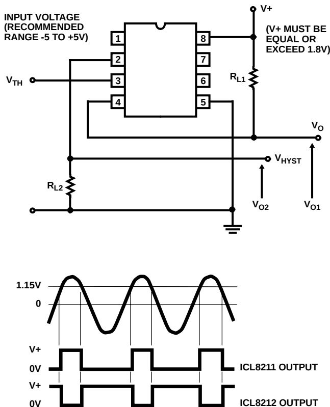
FIGURE 21. VOLTAGE LEVEL DETECTION
