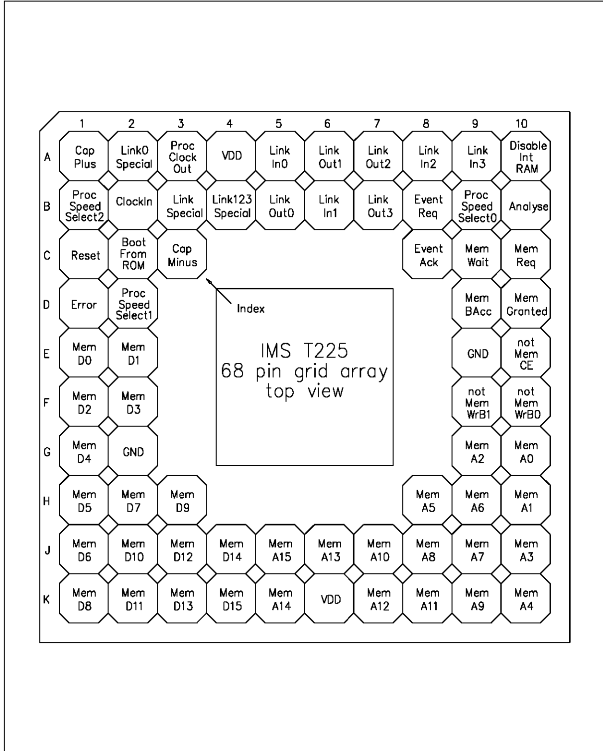
Figure 9.1 IMS T225 68 pin grid array package pinout
