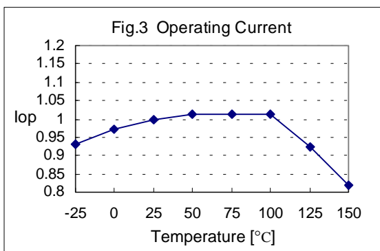
Figure 3. Operating Current
