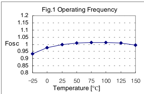
Figure 1. Operating Frequency
