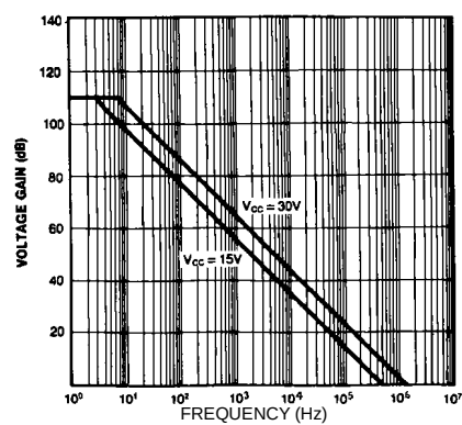
Fig. 5 OPEN LOOP FREQUENCY RESPONSE
